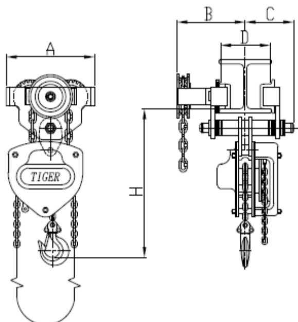
0.5t – 2.0t & 3.0t single bar geared trolley
