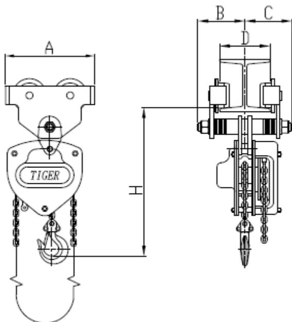
0.5t – 2.0t & 3.0t single bar plain trolley
